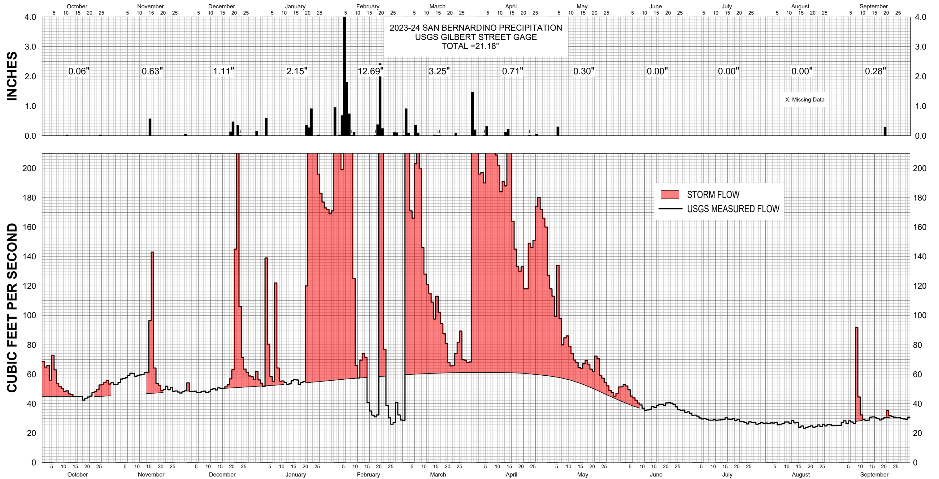
DISCHARGE OF SANTA ANA RIVER AT RIVERSIDE NARROWS & SAN BERNARDINO PRECIPITATION WATER YEAR 2023-24
