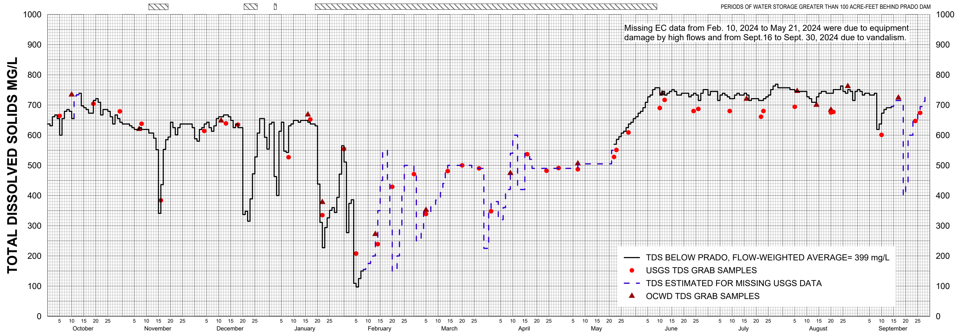
DISSOLVED SOLIDS IN SANTA ANA RIVER BELOW PRADO DAM WATER YEAR 2023-24
