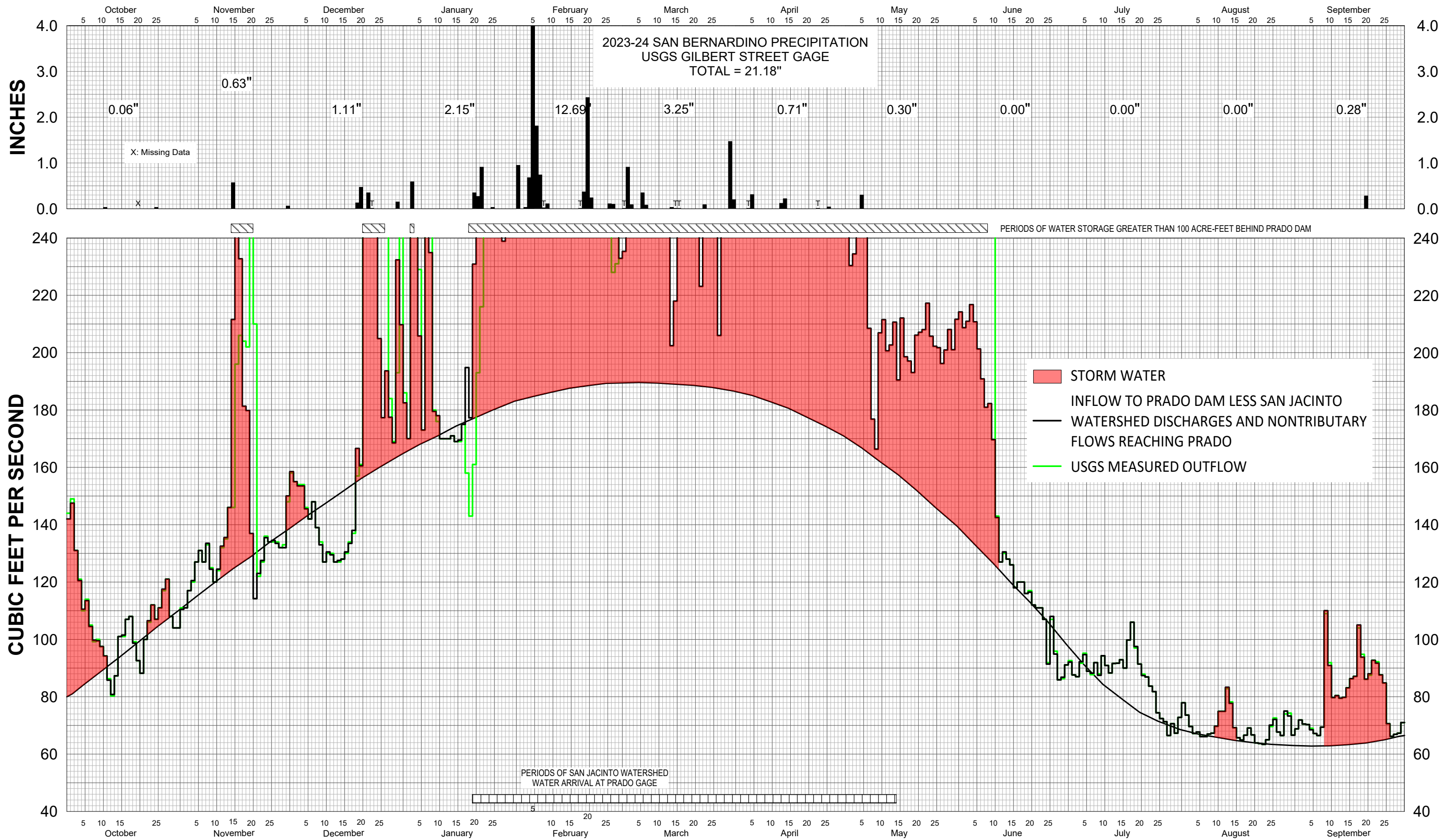
DISCHARGE OF THE SANTA ANA RIVER AT PRADO DAM & SAN BERNARDINO PRECIPITATION WATER YEAR 2023-24
