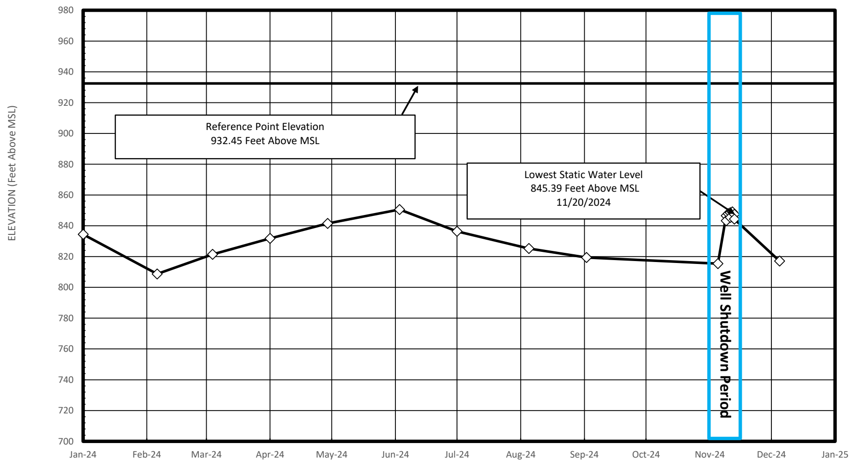
FIGURE 2 GROUNDWATER SURFACE ELEVATIONS 1S/4W-29H01S FLUME NO. 2 WELL 2024
