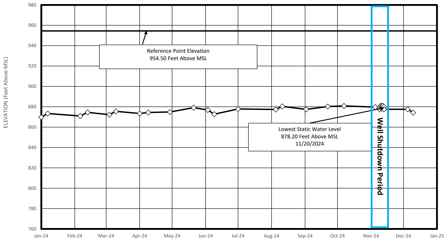
FIGURE 1 GROUNDWATER SURFACE ELEVATIONS 1S/4W-21Q03S JOHNSON NO. 1 WELL 2024
