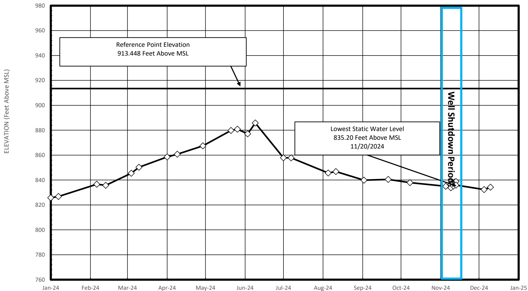
FIGURE 3 GROUNDWATER SURFACE ELEVATIONS 1S/4W-29Q01S FLUME NO. 5 WELL 2024
