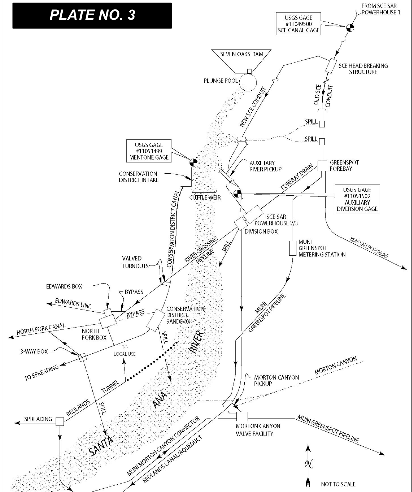
schematic of Water Control Features and Gages in the Santa Ana River Canyon
